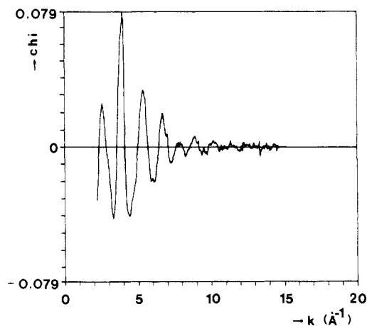
Figure 8. Raw EXAFS of the supported clusters formed from \text{Os}_3(\text{CO})_{12} and \gamma\text{-Al}_2\text{O}_3 after decomposition in He at 150 \text{ }^\circ\text{C} .
