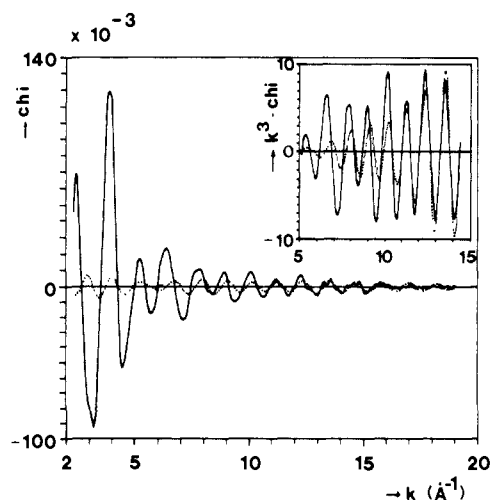
Figure 4. EXAFS of \text{Os}_3(\text{CO})_{12} (solid line) and calculated Os-Os shell ( N = 2 , R = 2.88 \text{ \AA} , \Delta\sigma^2 = -0.001 \text{ \AA}^2 relative to Pt foil) (dotted line).
