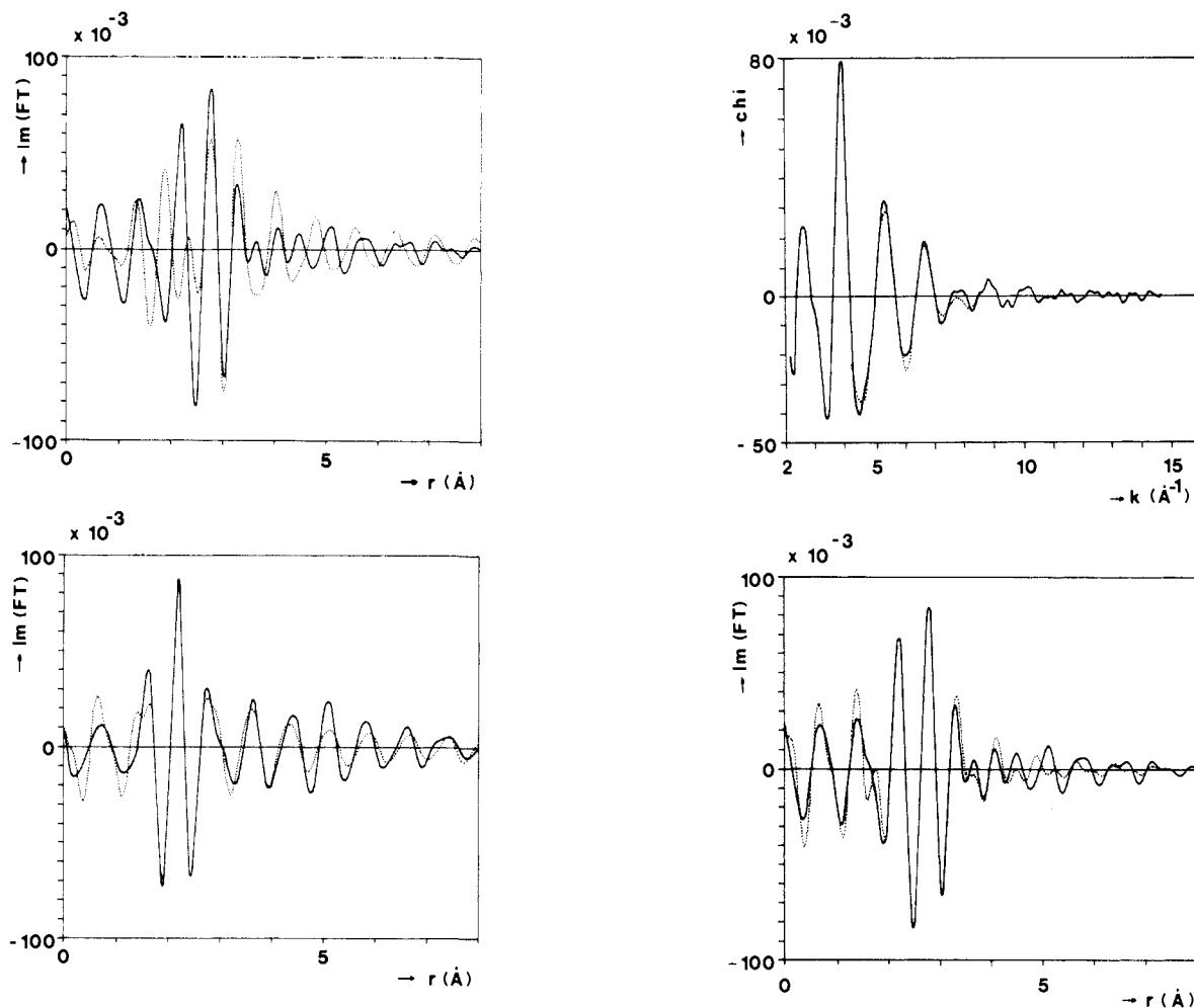
Figure 9. k^1 Fourier transforms ( \Delta k = 4.2\text{--}8.5 \text{ \AA}^{-1} ; Os-O phase corrected) of (a, top) decomposed cluster data (solid line) and calculated Os-CO shell ( N = 2.8 , R_{\text{Os-C}} = 1.91 \text{ \AA} , R_{\text{Os-O}} = 3.05 \text{ \AA} , \Delta\sigma^2 = 0 \text{ \AA}^2 relative to \text{Os}_3(\text{CO})_{12} ) (dotted line) and (b, bottom) decomposed cluster data minus Os-CO shell (solid line) and calculated Os- \text{O}_{\text{support}} shell ( N = 3 , R = 2.17 \text{ \AA} , \Delta\sigma^2 = -0.0025 \text{ \AA}^2 relative to \text{Na}_2\text{Pt}(\text{OH})_6 ) (dotted line).
