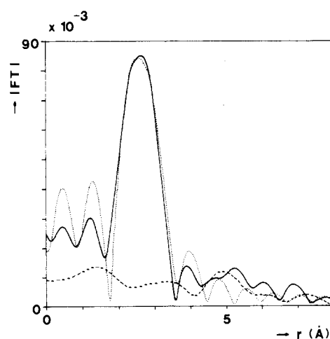
Figure 10. Experimental results characterizing the decomposed clusters on \gamma\text{-Al}_2\text{O}_3 (solid line) and the sum of the calculated Os-CO and Os- \text{O}_{\text{support}} shells (dotted line) (a, top) in k space, (b, middle) in r space (imaginary parts, \Delta k = 4.2\text{--}8.5 \text{ \AA}^{-1} , Os-O phase corrected), and (c, bottom) in r space (magnitude, \Delta k = 4.2\text{--}8.5 \text{ \AA}^{-1} , Os-O phase corrected). Also shown in (c) is the magnitude of the difference between experimental and calculated results ( \Delta k = 4.5\text{--}7.5 \text{ \AA}^{-1} , Os-O phase corrected) (dashed line).
